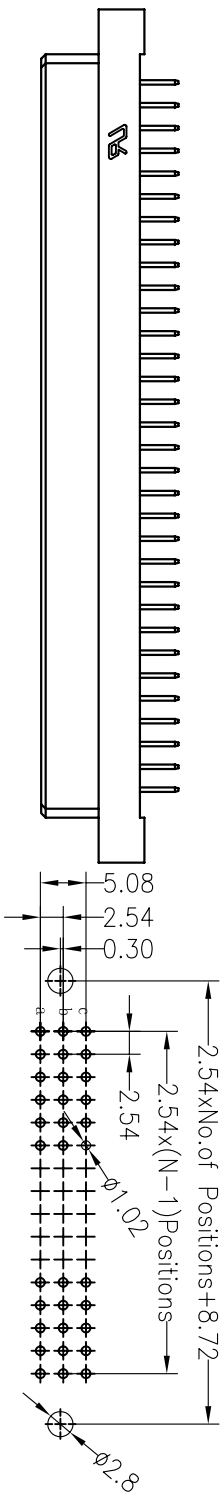
Recommended P.C.B Layout (Top Side) (PCB BOARD TOLERANCE ±0.05)
