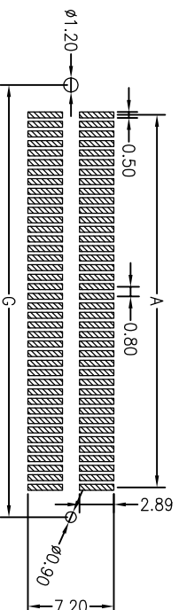
PCB LAYOUT
